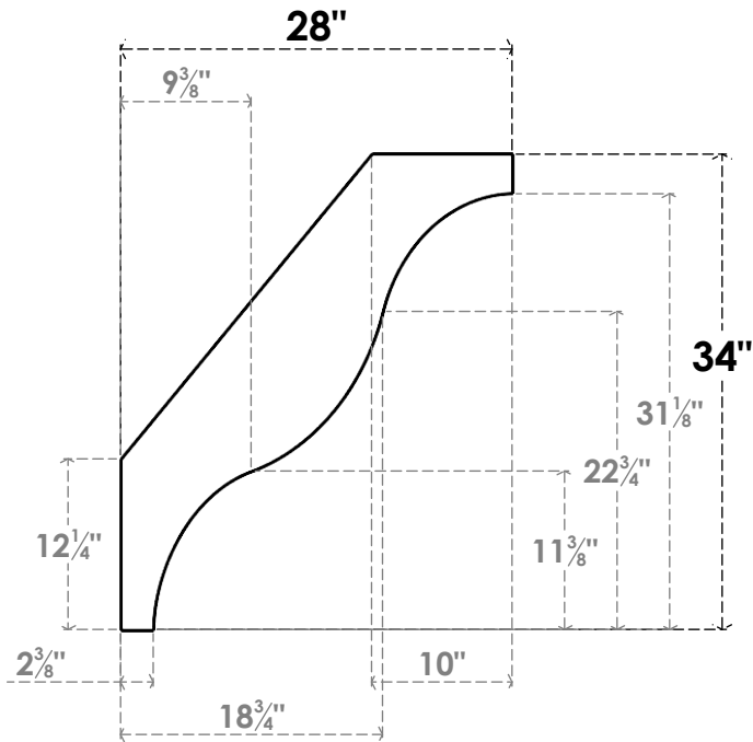
SIDE PROFILE
